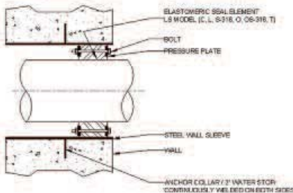
LINK-SEAL® MODULAR SEALS WITH MODEL WS STEEL WALL SLEEVES MANUFACTURED BY PIPELINE SEAL & INSULATOR, INC. HOUSTON, TEXAS, U.S.A. TEL: 800-423-2410 EMAIL: INFO@PSI.COM
