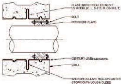
LINK-SEAL® MODULAR SEALS WITH CENTURY-LINE® SLEEVES MANUFACTURED BY PIPELINE SEAL & INSULATOR, INC. HOUSTON, TEXAS, U.S.A. TEL: 800-423-2410 EMAIL: INFO@PSI.COM
