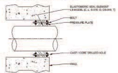
LINK-SEAL® MODULAR SEALS WITH CAST OR CORE DRILLED WALL OPENING MANUFACTURED BY PIPELINE SEAL & INSULATOR, INC. HOUSTON, TEXAS, U.S.A. TEL: 800-423-2410 EMAIL: INFO@PSI.COM
