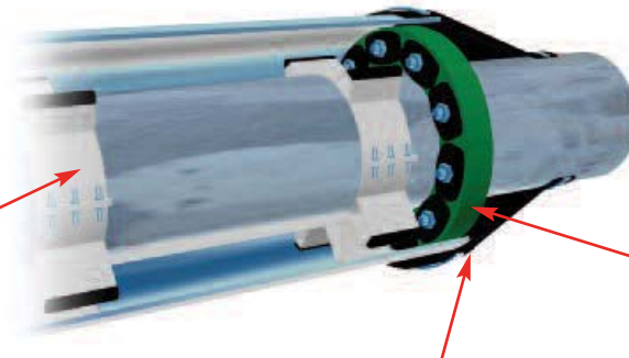
Link-Seal® modular seals with Centering Blocks
